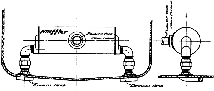
FIG. 19.—Underwater Exhaust.
